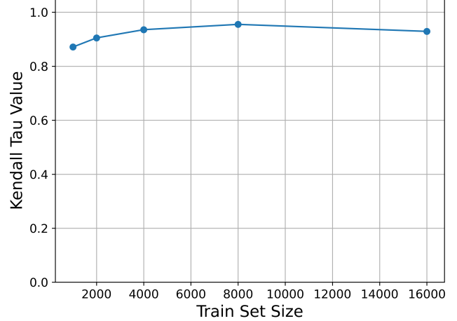
Figure 1: Kendall Tau correlation between the influence rankings produced by the highest-loss test sample used in prior work [1] and the proposed median-based aggregation across different training set sizes.
