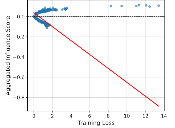
(b) ADULT TracIn
